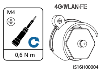
Figure 5-12 Installation des composants antivol du dongle intelligent
